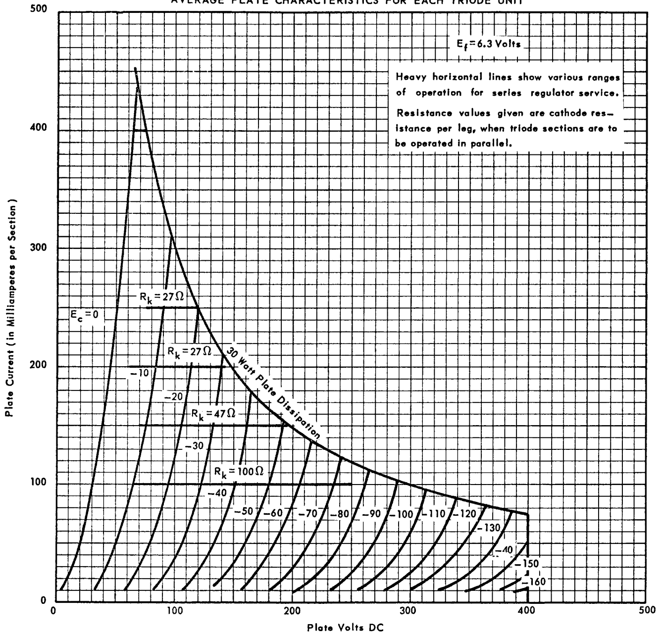
AVERAGE PLATE CHARACTERISTICS FOR EACH TRIODE UNIT
